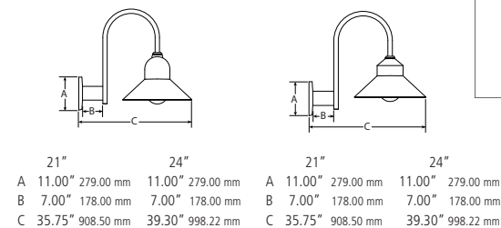
WALL BRACKET WB21, WB24
