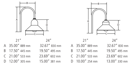
ARM MOUNT SINGLE AM(**)ISF3/ISF4
