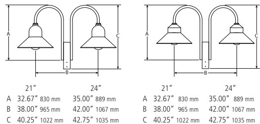
ARM MOUNT 2 @ 180° AM(**)ESF3-2180
